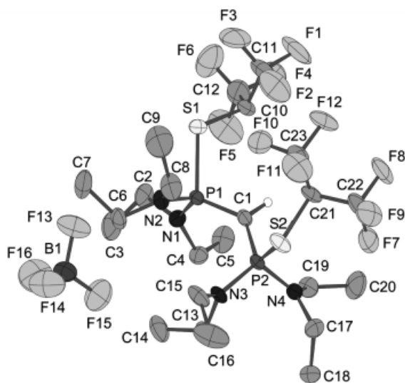
Figure 3. Perspective view and labeling scheme for the molecule 18 ; selected bond lengths [pm] and angles ^\circ : P(1)–N(1) 163.6(3), P(1)–C(1) 169.6(4), C(1)–P(2) 169.7(4), P(1)–S(1) 212.72(14), S(1)–C(10) 182.5(4), N(1)–C(2) 148.2(5), C(10)–C(11) 152.2(6); C(1)–P(1)–N(2) 116.21(19), C(1)–P(1)–S(1) 111.42(14), N(1)–P(1)–S(1) 107.61(13), N(1)–P(1)–N(2) 108.99(17), P(1)–C(1)–P(2) 129.2(2), P(1)–S(1)–C(10) 111.86(15)
