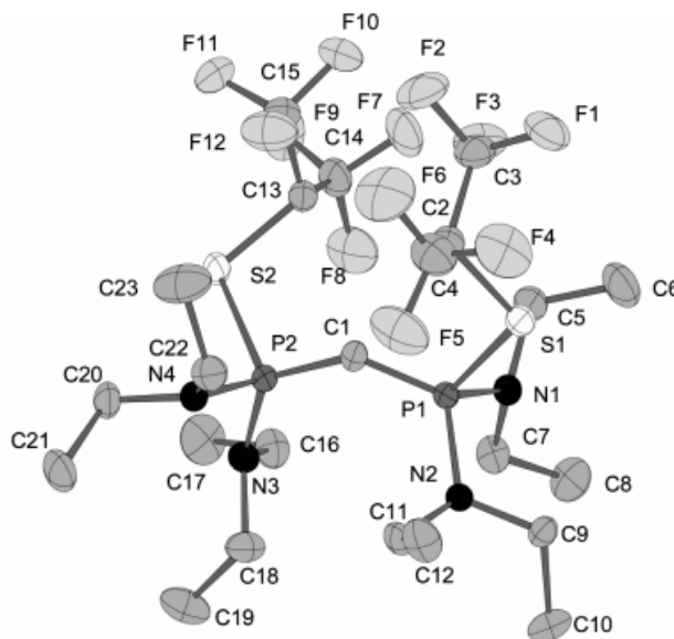
Figure 2. Perspective view and labeling scheme for the molecule 15 (H atoms are omitted for clarity); selected bond lengths [pm] and angles [°]: P(1)–N(1) 167.32(12), P(1)–C(1) 162.57(15), C(1)–P(2) 162.60(15), P(1)–S(1) 217.60(5), S(1)–C(2) 180.40(16), N(1)–C(5) 147.81(19), C(2)–C(3) 152.1(2); C(1)–P(1)–N(1) 122.84(7), C(1)–P(1)–S(1) 108.73(5), N(1)–P(1)–N(2) 101.47(6), N(1)–P(1)–S(1) 98.12(5), P(1)–C(1)–P(2) 139.52(9), P(1)–S(1)–C(2) 101.81(5)
