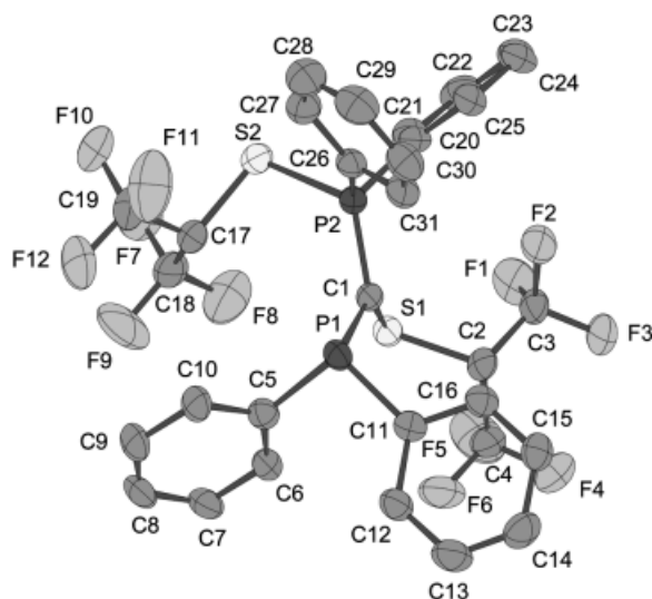
Figure 4. Perspective view and labeling scheme for the molecule 21 ; selected bond lengths [pm] and angles [°]: P(1)–C(1) 181.4(5), C(1)–P(2) 170.4(5), P(2)–S(2) 215.55(19), C(1)–S(1) 176.8(5), P(1)–C(5) 183.1(5), P(2)–C(20) 181.3(5); P(1)–C(1)–P(2) 117.6(3), C(1)–P(1)–C(5) 106.2(2), P(1)–C(1)–S(1) 125.5(3), P(2)–C(1)–S(1) 113.4(3), C(1)–P(2)–S(2) 117.22(18), C(1)–P(2)–C(20) 116.0(2)
